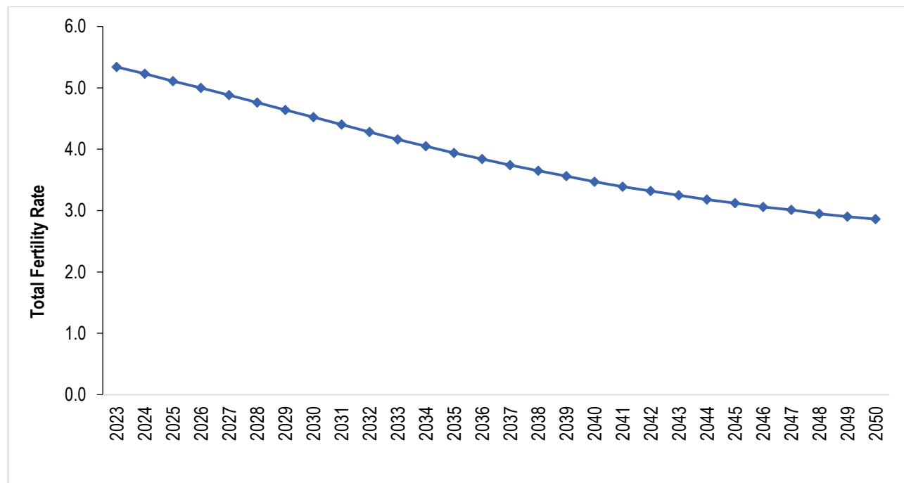
Figure 3.2: Projected Total Fertility Rates; Songwe Region, 2023 – 2050
