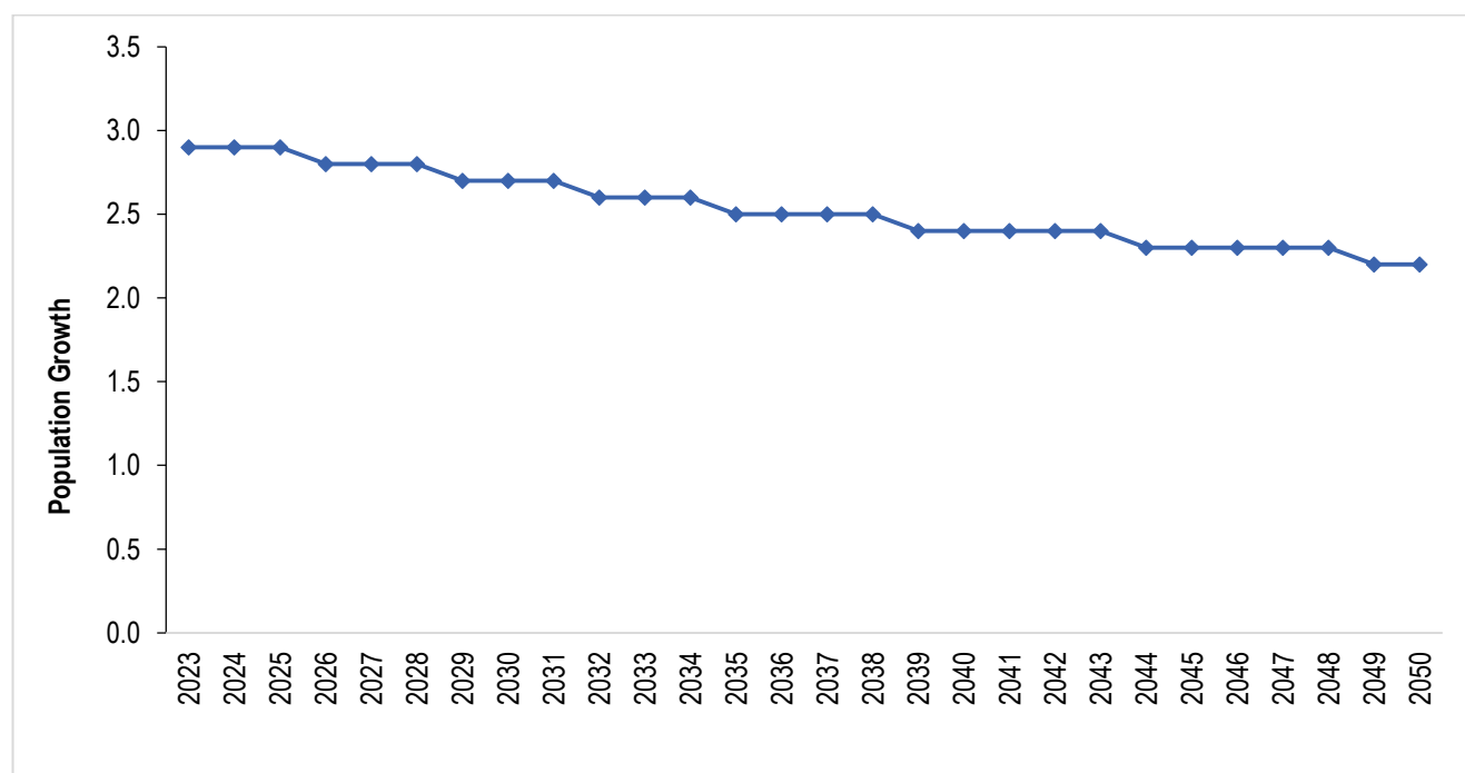
Figure 3.1: Projected Population Growth Rates; Songwe Region; 2023 – 2050
