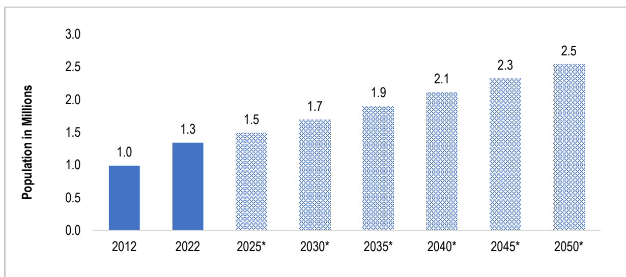
Figure 1.1: Population Trends; Songwe Region, 2012 – 2050
