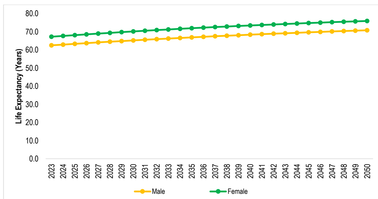
Figure 2. 2: Mortality Assumptions - Life Expectancy at Birth; Songwe Region, 2023 – 2050
