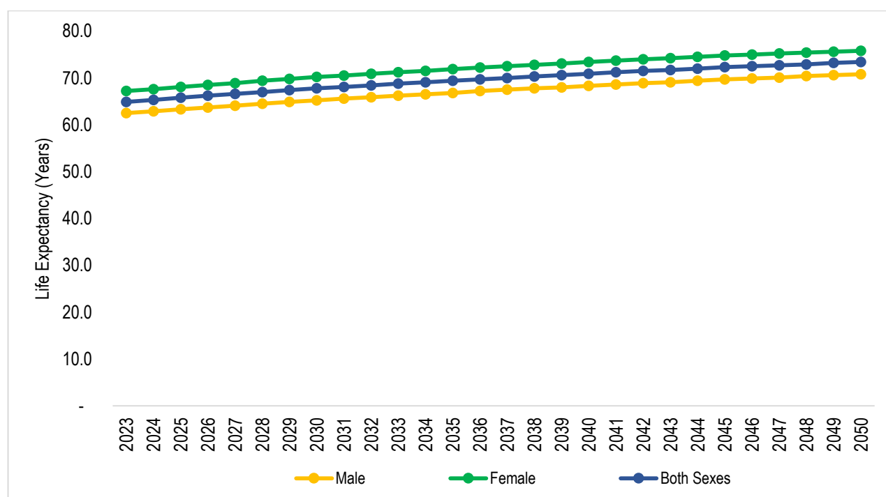
Figure 3.3: Projected Life Expectancy at Birth by Sex; Songwe Region, 2023 – 2050
