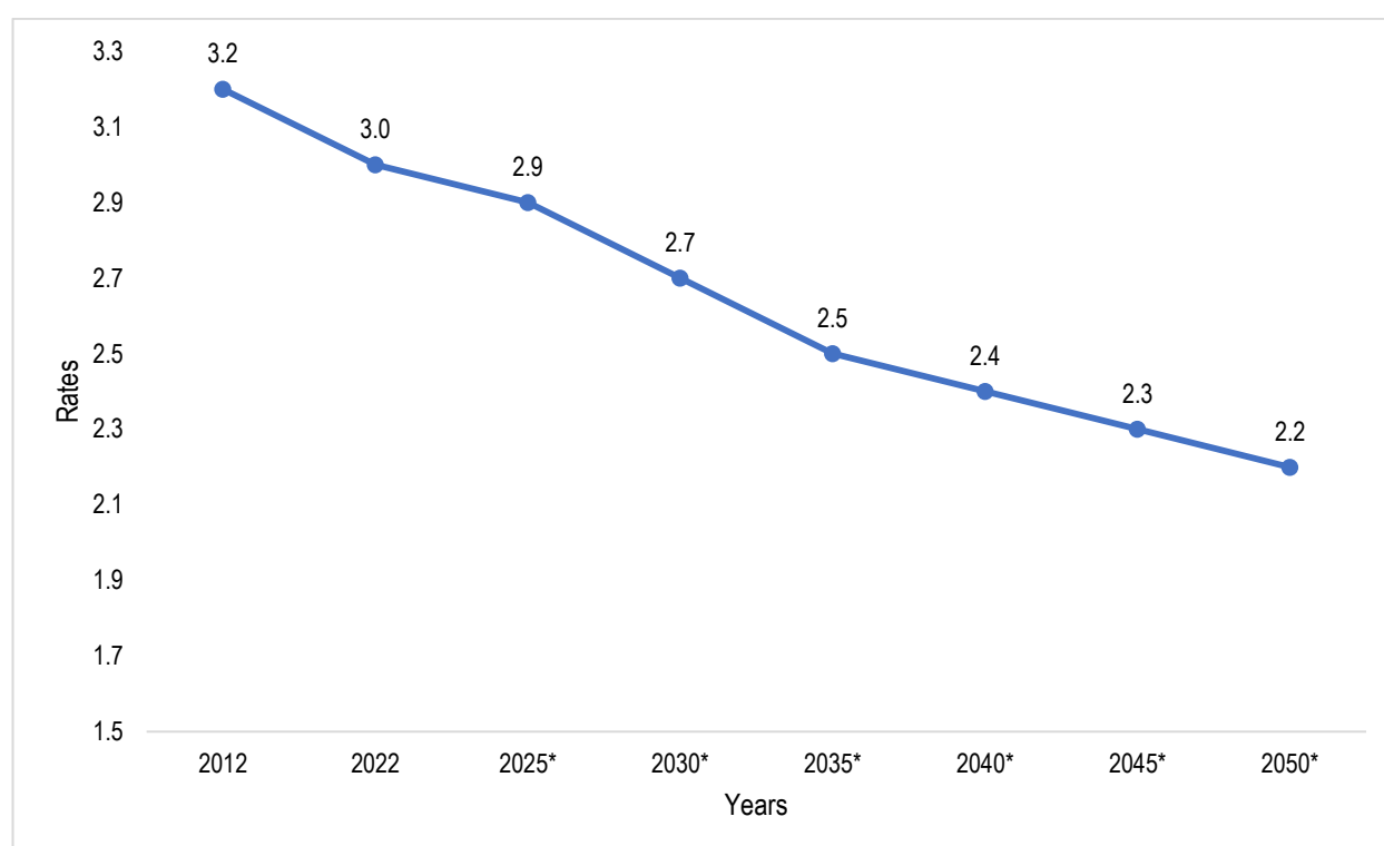
Figure 1.2: Average Annual Inter-Censal Population Growth Rates; Songwe Region, 2012–2050
