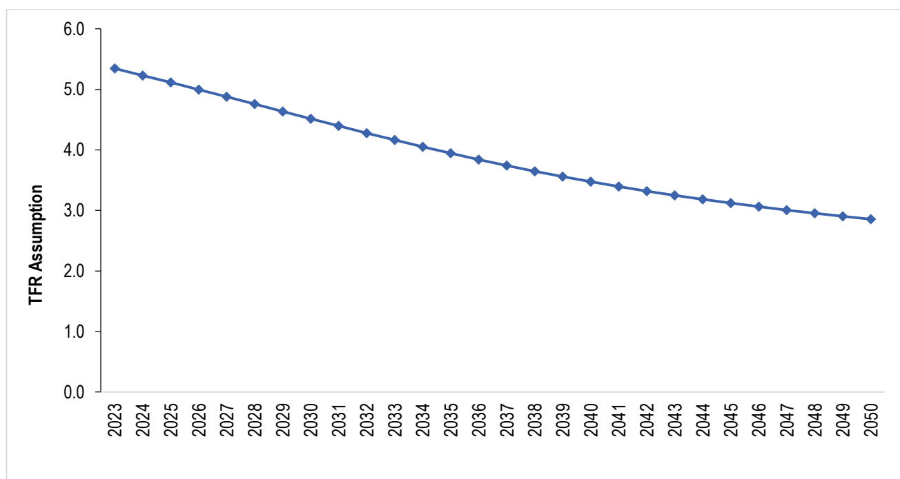
Figure 2.1: Fertility Assumptions; Songwe Region, 2023 – 2050
