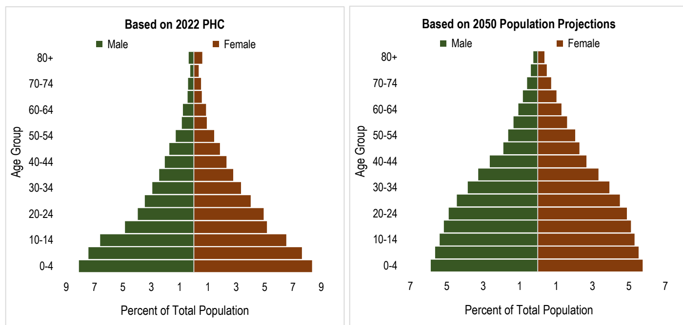
Figure 1.4: Projected Population Pyramid for Five Year Age Groups; Songwe Region, 2022 and 2050
